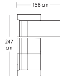
A2002 - 2 SEAT 1 ARM A2002 SEATING CORNER
